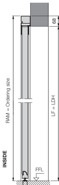
Steel side door Block frame Profile type 2 Fitted behind the opening
