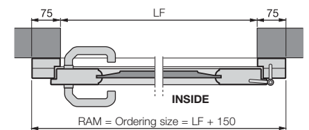
Timber side door Fitted behind the opening
